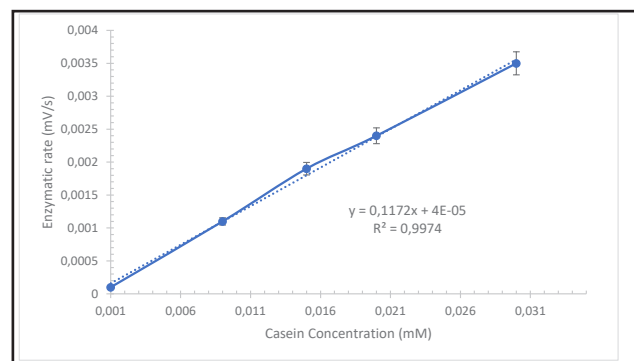
Fig. 4. Calibration curve obtained with a biosensor Peptidase _C1 with enzyme immobilized
