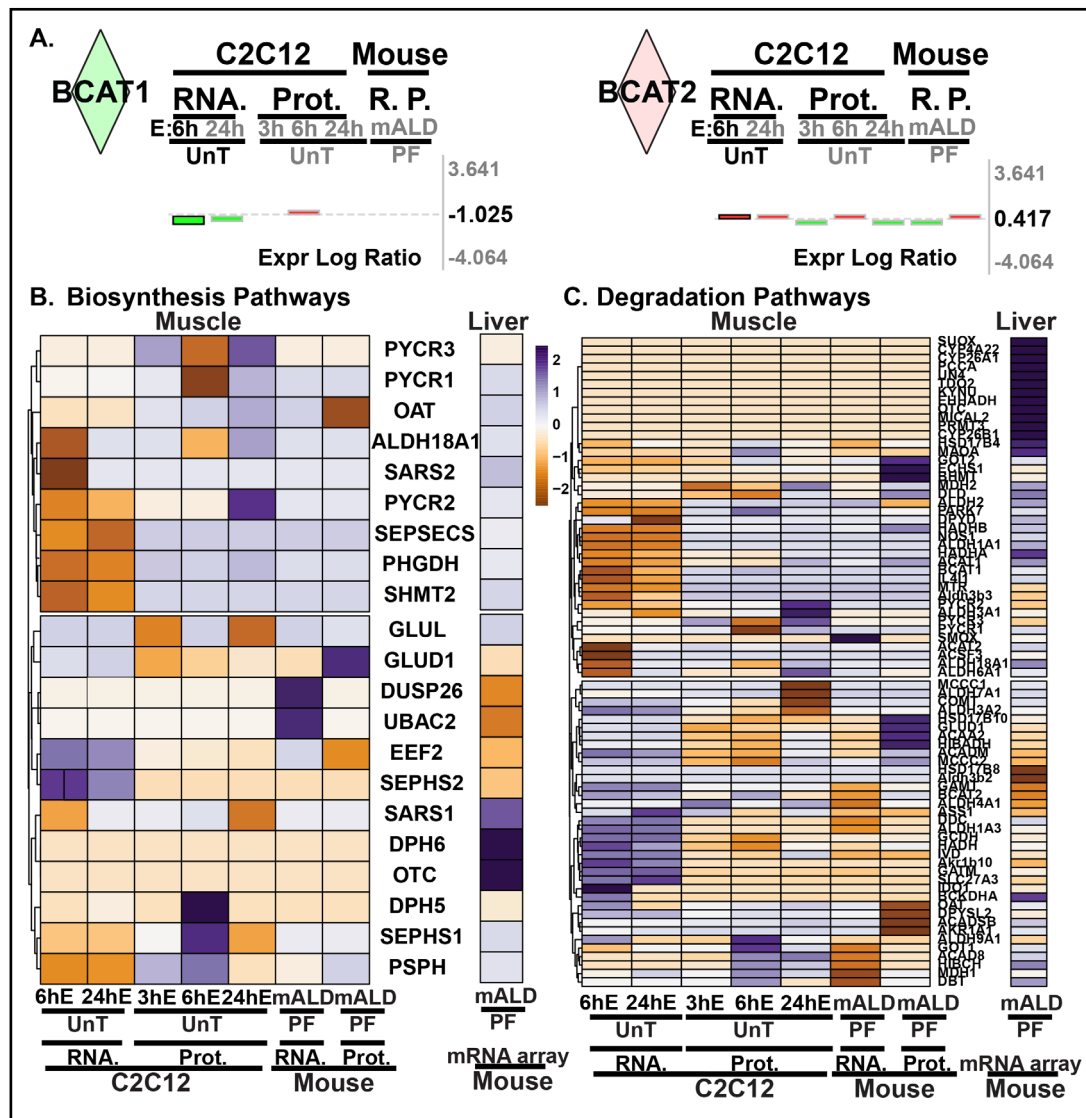
Fig. 4. Ethanol induced alterations in amino acid metabolism enzyme expression. (A). Log fold change expression levels of BCAT1 and BCAT2 in the transcriptome and proteome in C2C12 myotubes and mALD versus untreated controls and PF mice. (B). Heatmap of differentially expressed genes regulating non-essential amino acid biosynthesis pathways. (C). Heatmap of differentially expressed genes regulating proteino-genic (essential and non-essential) amino acid degradation pathways. EtOH/E: ethanol; HMB: \beta -hydroxy- \beta -methyl butyrate; UnT: untreated controls; PF: pair-fed mice; mALD: mouse model of ALD; Prot, P.: proteomics; RNA, R.: RNAseq. N = 3 biological replicates for untreated and ethanol-treated myotubes; N = 4 mice in mALD and PF groups. Significance for proteomics and transcriptomics expression levels for cells and tissue (muscle and liver) was limited to p < 0.05 . Significance for pathway enrichment analysis was limited to -\log(p\text{-value}) \geq 1.3 .
