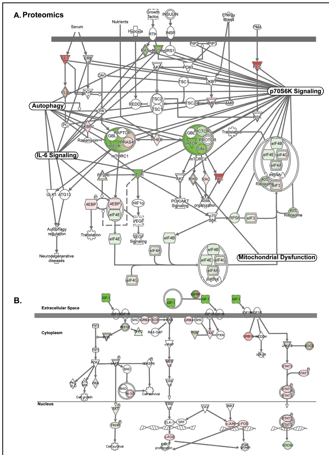
Fig. 2. Regulatory networks in ethanol treated myotubes identify HMB targets. (A). Integrated network of the proteome from ethanol-treated myotubes of HMB targets- mTORC1 signaling with nodes including mitochondrial dysfunction, p70S6k signaling, AMPK signaling, and senescence pathways connected via shared molecules. (B). Integrated network of IGF-1 signaling pathway in ethanol treated myotubes. N= 3 biological replicates for untreated and ethanol-treated myotubes. Significance for proteomics and transcriptomics expression levels for cells was limited to p < 0.05 . Significance for pathway enrichment analysis was limited to -\log(p\text{-value}) = > 1.3 .
