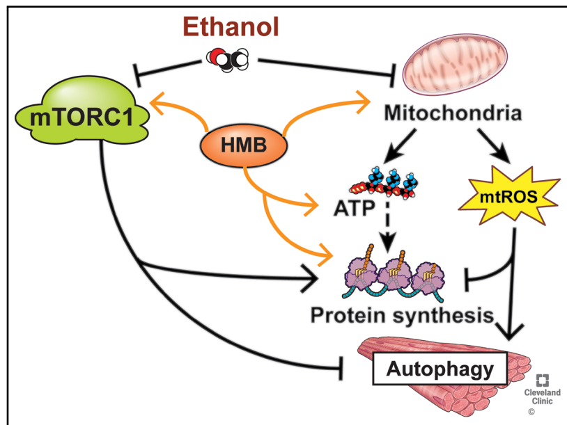
Fig. 11. Graphical abstract: Ethanol induced perturbations in skeletal muscle that are responsive to HMB supplementation.
