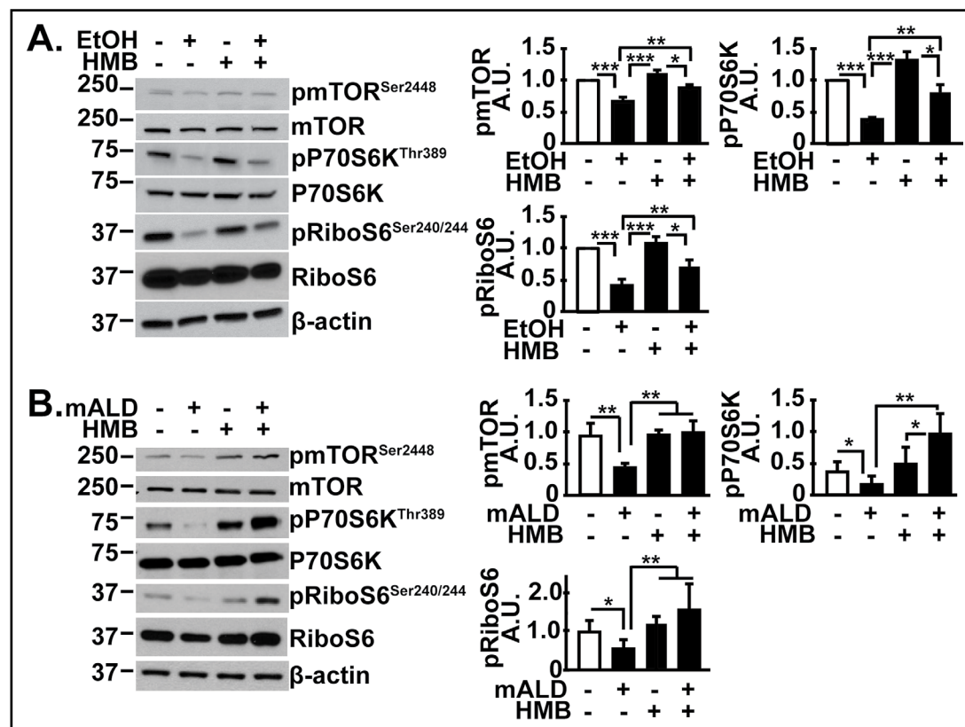
Fig. 5. HMB reversed impaired mTORC1 signaling in alcoholic liver disease. Representative immunoblots and densitometry of phosphorylated mTOR (Ser2448) and signaling response to mTORC1 activation (phosphorylation of P70S6 kinase and ribosomal S6 protein) shown. (A) Differentiated C2C12 myotubes that were untreated or treated with 100 mM ethanol, with or without 50 μM HMB. (B) Studies in gastrocnemius muscle from PF or mALD mice with or without HMB. All data expressed as mean±SD from at least three biological replicates for experiments in C2C12 myotubes; n=6 mALD and n=4 PF mice in each group. * p<0.05; ** p<0.01, *** p<0.001. EtOH: ethanol; HMB β-hydroxy-β-methyl butyrate; UnT: untreated controls; PF: paired mice; mALD: mouse model of ALD.
