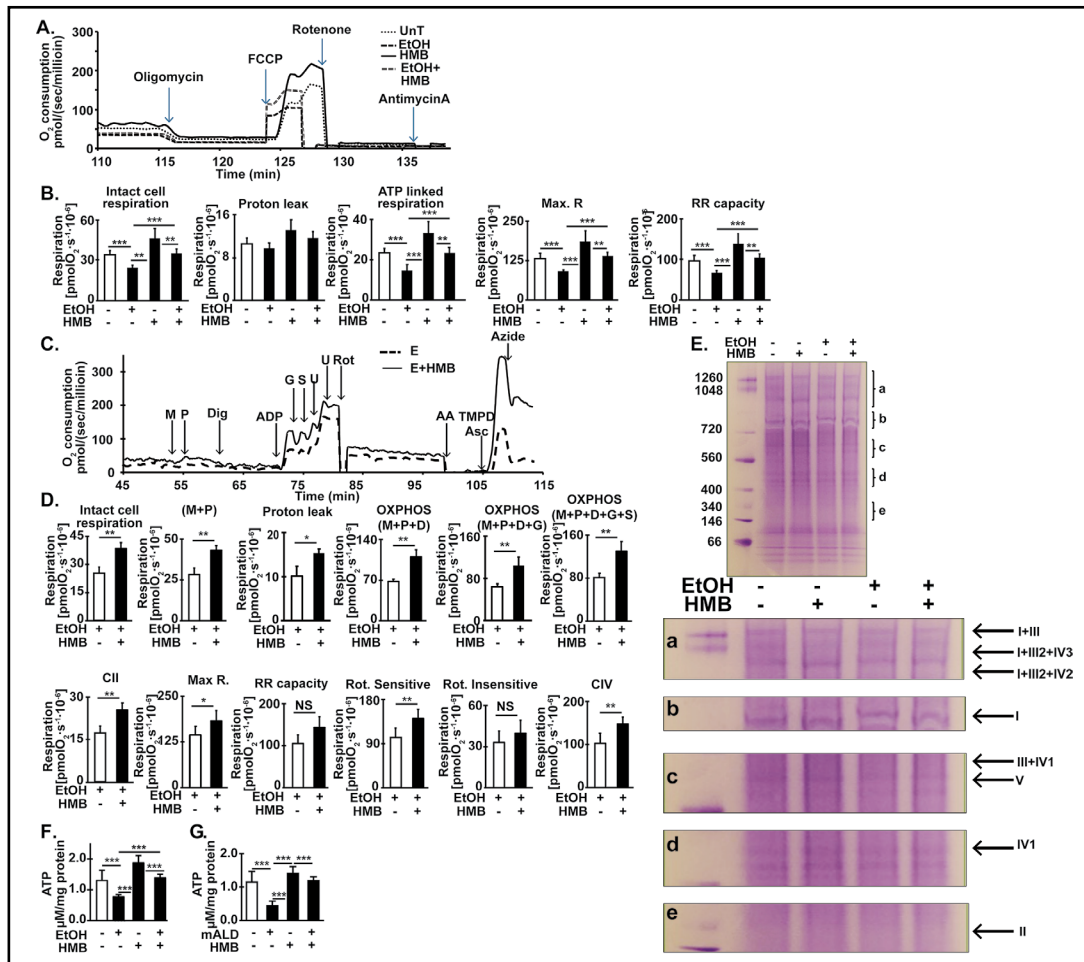
Fig. 6. Ethanol impairs and HMB restores mitochondrial respiration in differentiated C2C12 myotubes and ATP content in muscle from mice model of ALD. (A) Representative tracings of high-resolution respirometry to quantify intact cell respiration of differentiated C2C12 myotubes. After initial stabilization, ATP synthetase inhibitor, oligomycin (O) was added, and oxygen consumption quantified to determine the oligomycin-sensitive and -insensitive respiration. Uncoupler of oxidative phosphorylation, FCCP (U) at 0.5 \mu M increments was then added to quantify maximum respiratory capacity. This was followed by rotenone (R) 375 nM final concentration, to inhibit complex I of the ETC, and then 2.5 \mu M antimycin A (Aa), which inhibits complex III, was added to determine non-mitochondrial respiration. (B) Intact, non-permeabilized C2C12 myotubes in basal DMEM medium were either untreated or treated with 100 mM ethanol for 6h with and without 50 \mu M HMB for 6h. Basal cell respiration, proton leak, ATP-linked respiration, maximum respiratory capacity (Max. Resp.) from the response to FCCP and reserve respiratory capacity (Reserve Resp.) were measured. (C) Representative tracings of high-resolution respirometry to quantify respiration of permeabilized differentiated C2C12 myotubes. After initial stabilization, 2 mM malate (M) and 2.5 mM pyruvate (P) were added. This was followed by 4.1 mM digitonin (Dig) to permeabilize the cell membrane without losing the integrity of cells or mitochondria for permitting entry of mitochondrial substrates inside the cells; 2.5 mM ADP (D); 10 mM glutamate (G); 10 mM succinate (S); 2 mM increments of FCCP (U) for measuring maximum respiration; 375 nM rotenone (R); 125 nM antimycin A (Aa); 2 mM ascorbate and 2 mM TMPD (tetramethyl p-phenylene diamine) (AT) to test complex IV activity; 50 mM sodium azide (Az) to inhibit complex IV activity. (D) Oxygen consumption was measured in intact non-permeabilized C2C12 myotubes treated with 100 mM ethanol with and without HMB in mitochondrial respiration buffer followed by digitonin permeabilization and ETC complex specific substrates and inhibitors sequentially in the concentrations as stated above. Intact cell respiration, oxidative phosphorylation (OXPHOS) in response to M, P, D, G and S, and Max. R and RR capacity (response to U) were quantified. Rotenone-sensitive and -insensitive respiration and complex II and IV function were measured. (E) Blue native gel electrophoresis of isolated mitochondria to evaluate mitochondrial supercomplex assembly. (F) Total ATP content in C2C12 myotubes either untreated or treated with 100mM ethanol for 6hours with and without 50 \mu M HMB. (G) ATP content in gastrocnemius muscle from mALD mice with and without HMB compared to that from PF mice with and without HMB. * p < 0.05 ; ** p < 0.01 , *** p < 0.001 . EtOH: ethanol; HMB \beta -hydroxy- \beta -methyl butyrate; UnT: untreated controls; PF: paired mice; mALD: mouse model of ALD.
