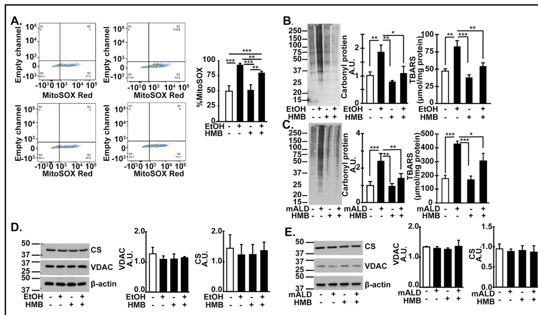
Fig. 7. Ethanol-induced increase in free radical generation is reversed by HMB. Studies in differentiated C2C12 myotubes treated with/without 100mM ethanol with/without 50 μM HMB for 6h. (A) Representative flow cytometry of myotubes gated for MitoSox fluorescence and percentage of MitoSox fluorescent cells. (B) Representative immunoblots of carbonylated proteins and densitometry, and TBARS in myotubes treated with/without 100mM ethanol with/without 50 μM HMB for 6h. (C) Representative immunoblots and densitometry of carbonylated proteins, and tissue concentration of TBARS in gastrocnemius muscle from mALD and PF mice treated with/without HMB. (D) Representative immunoblots and densitometry of voltage dependent anion channel (VDAC) and citrate synthase (CS) expression in myotubes as measures of mitochondrial mass. (E). Representative immunoblots of VDAC and CS in gastrocnemius muscle from PF mice and mALD and PF mice treated with and without HMB. All data expressed as mean±SD from at least three biological replicates for experiments in C2C12 myotubes and n=4 PF and n=6 mice. *p<0.05; **p<0.01; ***p<0.001. EtOH: ethanol, TBARS: thiobarbituric acid reactive substances; UnT: untreated controls; PF: pair-fed; mALD: mouse model of ALD.
