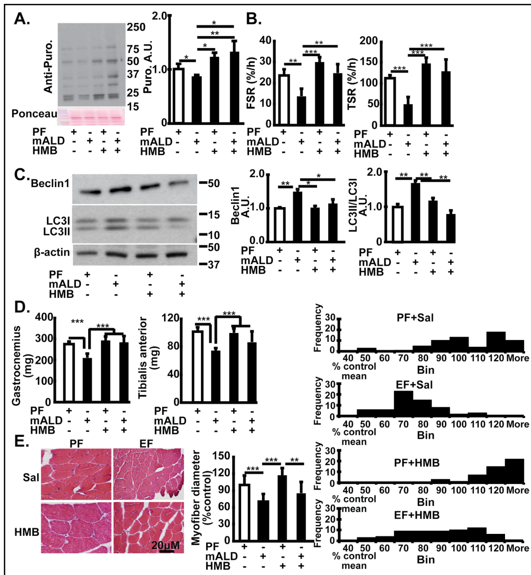
Fig. 10. Skeletal muscle responses to HMB in muscle from mice with ALD. (A). Representative immunoblots of incorporation of puromycin in ex vivo gastrocnemius muscle from PF mice and mALD treated with and without HMB. Densitometry of all blots in each lane. (B). Fractional and total synthesis rate of muscle protein in gastrocnemius muscle from PF mice and mALD above. (C). Representative immunoblots and densitometry of LC3 lipidation and Beclin 1 expression in mouse gastrocnemius muscle from mALD and PF mice with or without HMB. (D). Tissue weight (gm) of gastrocnemius and tibialis anterior muscles from mALD and PF mice treated with or without HMB. (E). Representative cross-sectional histological cryosections of gastrocnemius muscle oriented in the longitudinal direction from mALD and PF mice treated with or without HMB. All data expressed as mean±SD from n=4 PF mice and n= 6 mALD. * p<0.05; ** p<0.01, *** p<0.001. EtOH: ethanol; HMB β-hydroxy-β-methyl butyrate; UnT: untreated controls; PF: pair-fed; mALD: mouse model of ALD.
