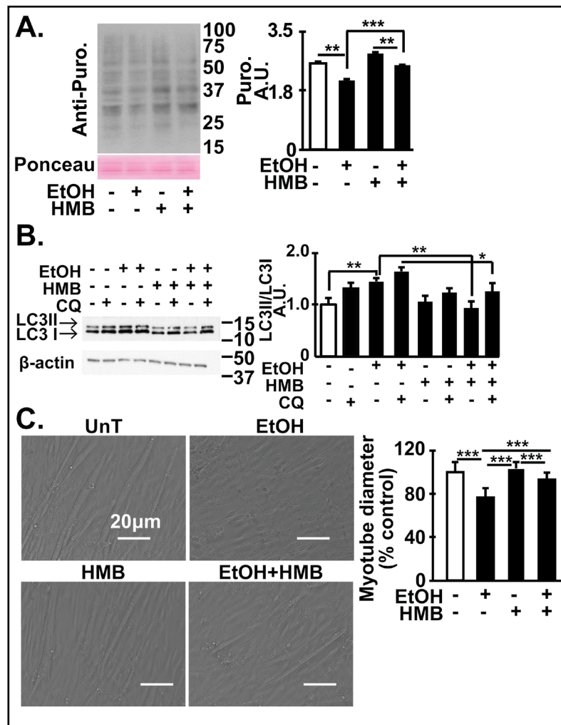
Fig. 9. Skeletal muscle dys-regulated proteostasis and ethanol-induced phenotype reversed by HMB. (A) Representative immunoblots and densitometry (for the indicated conditions) for puromycin incorporation in C2C12 myotubes that were untreated or treated with 100 mM ethanol with or without 50 \mu M HMB. (B) Representative immunoblots and densitometry of LC3 lipidation in differentiated C2C12 myotubes treated with 100 mM ethanol for 6h with and without 50 \mu M HMB. Chloroquine was used to determine autophagy flux. (C). Representative photomicrographs of C2C12 myotubes treated with and without ethanol and HMB. Mean diameter of at least 100 myotubes in each group. All data mean+SD from at least 3 biological replicates for myotubes and n=4 PF and n=6 mALD mice. *p<0.05; **p<0.01; ***p<0.001. EtOH: ethanol;
